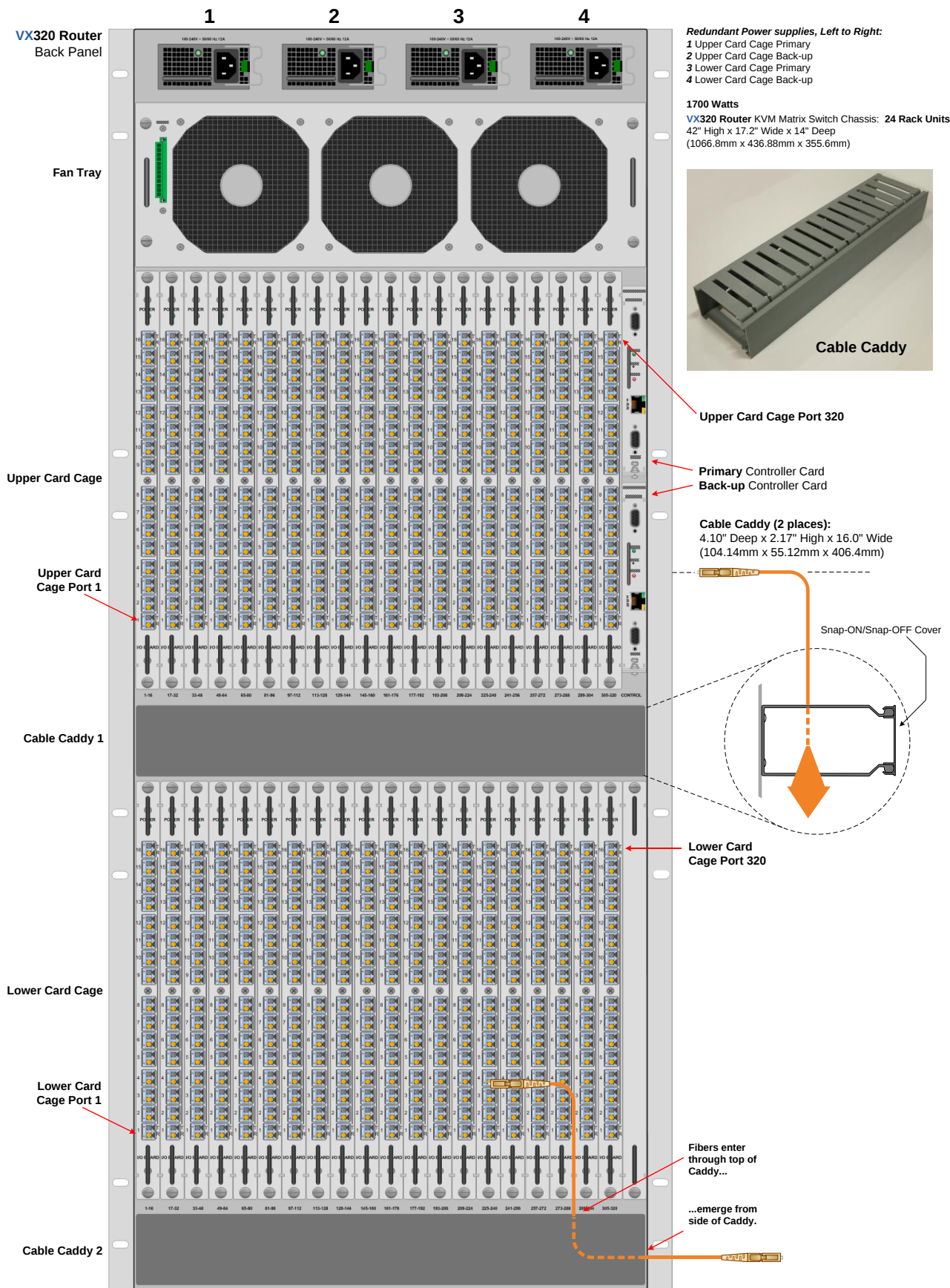
VX320 Matrix Switch – Rear View
