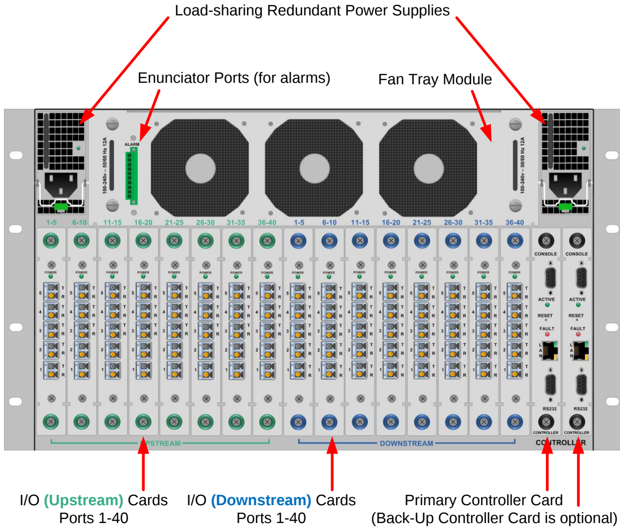
VX40 Matrix Switch – Rear View
