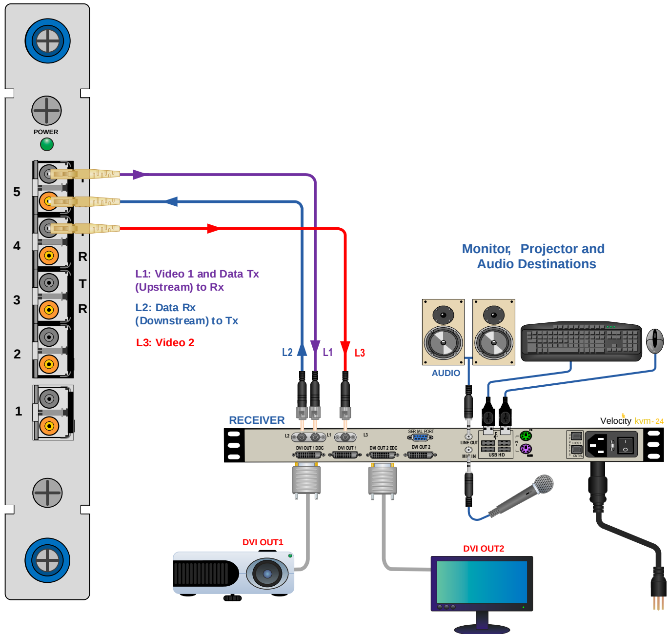
Connecting the Thinklogical VelocityKVM-24 Extender Receiver to the VX40/VX80
