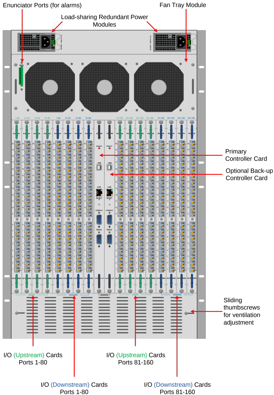
VX160 Matrix Switch – Rear View
