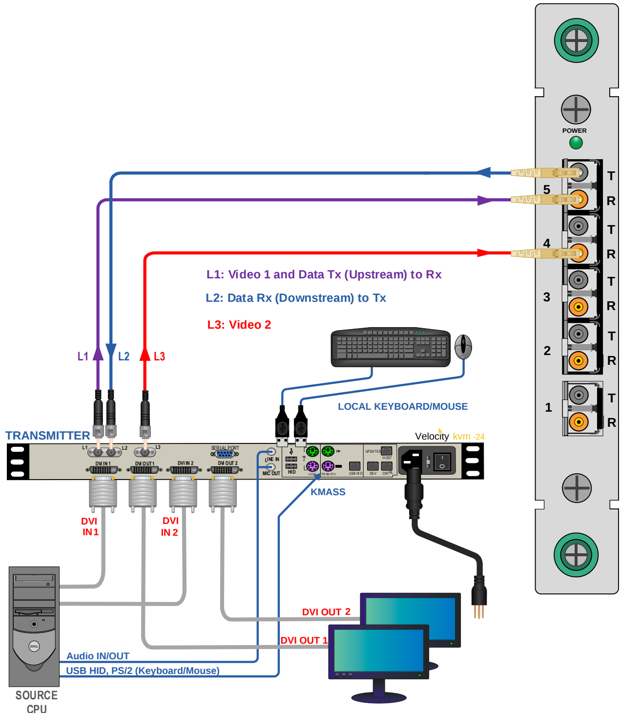
Connecting the Thinklogical VelocityKVM-24 Extender Transmitter to the VX40/VX80
