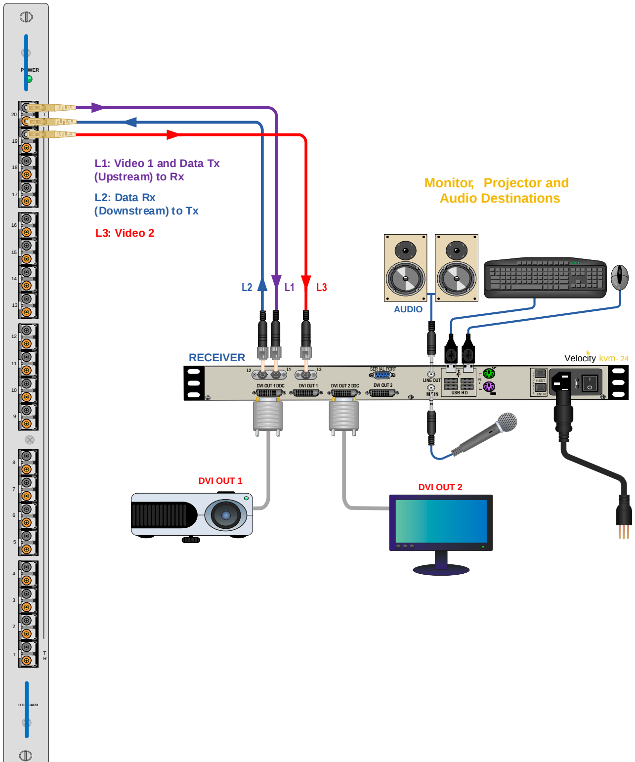
Connecting the Thinklogical VelocityKVM-24 Extender Receiver to the VX160
