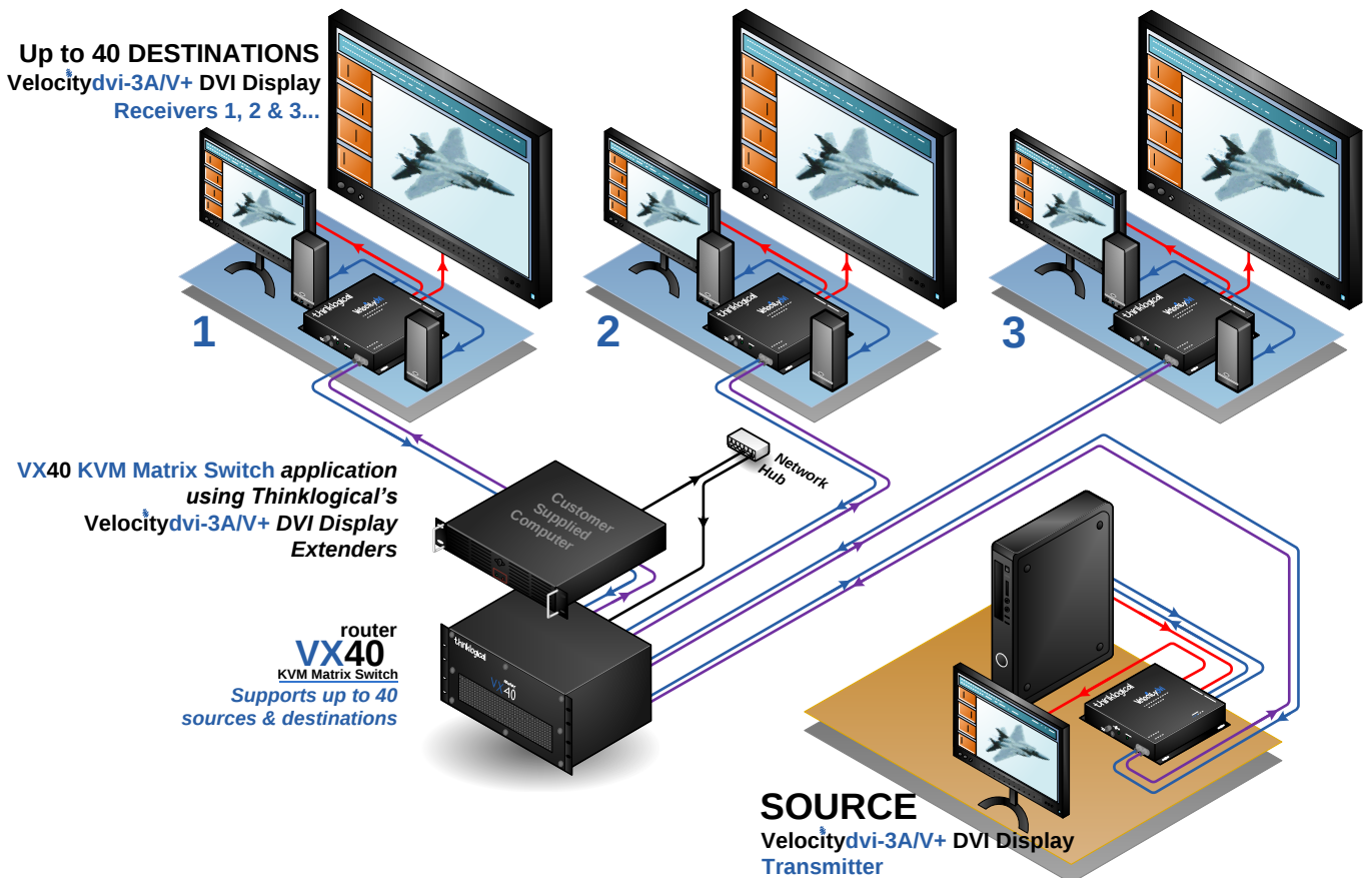
Typical VX40 Matrix Switch Application using VelocityDVI-3AV+ Extenders
