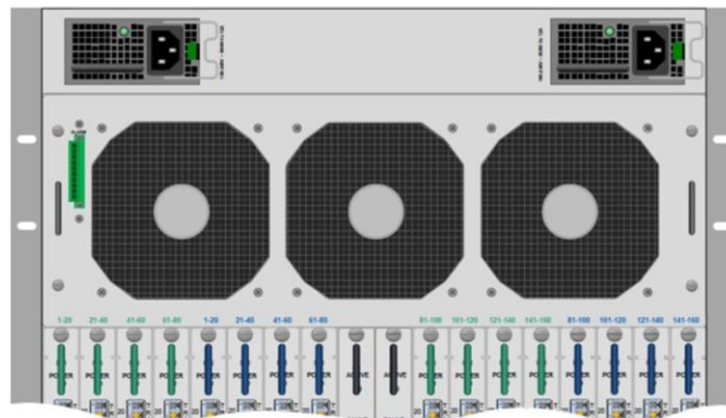
VX Matrix Switch Power Supplies and Fan Tray with Alarm Annunciator
