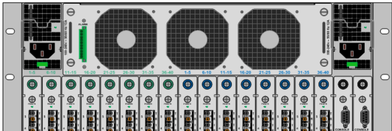
VX40 Input / Output Port Numbering
