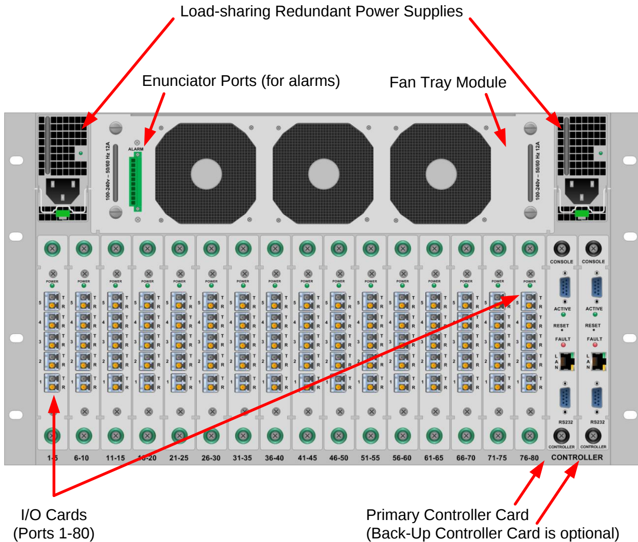
VX80 Matrix Switch – Rear View
