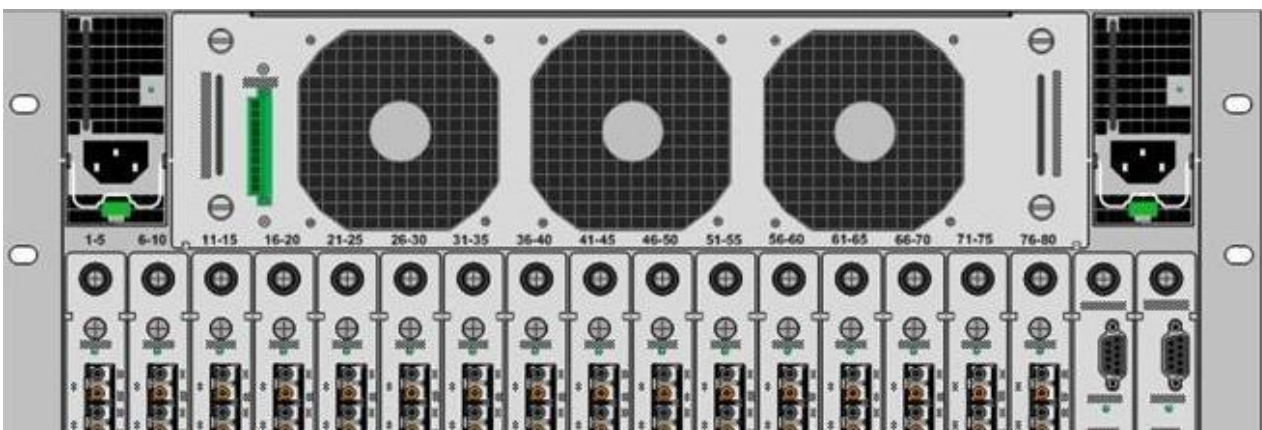
VX80 Input / Output Port Numbering
