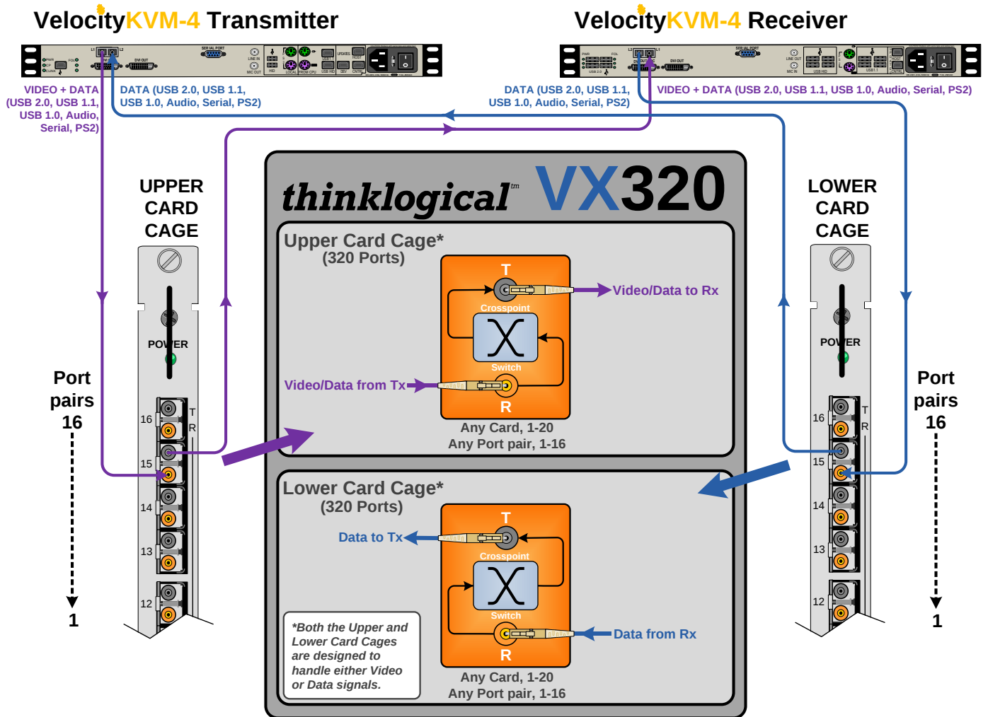
Connecting the Thinklogical VelocityKVM-4 Extender Transmitter and Receiver to the VX320
