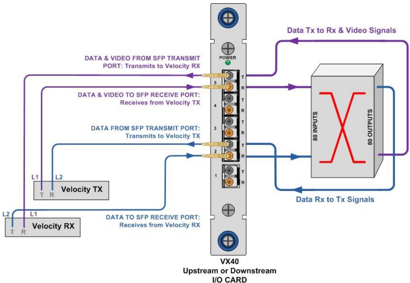
Figure 1: VX40 Input/Output Concept
