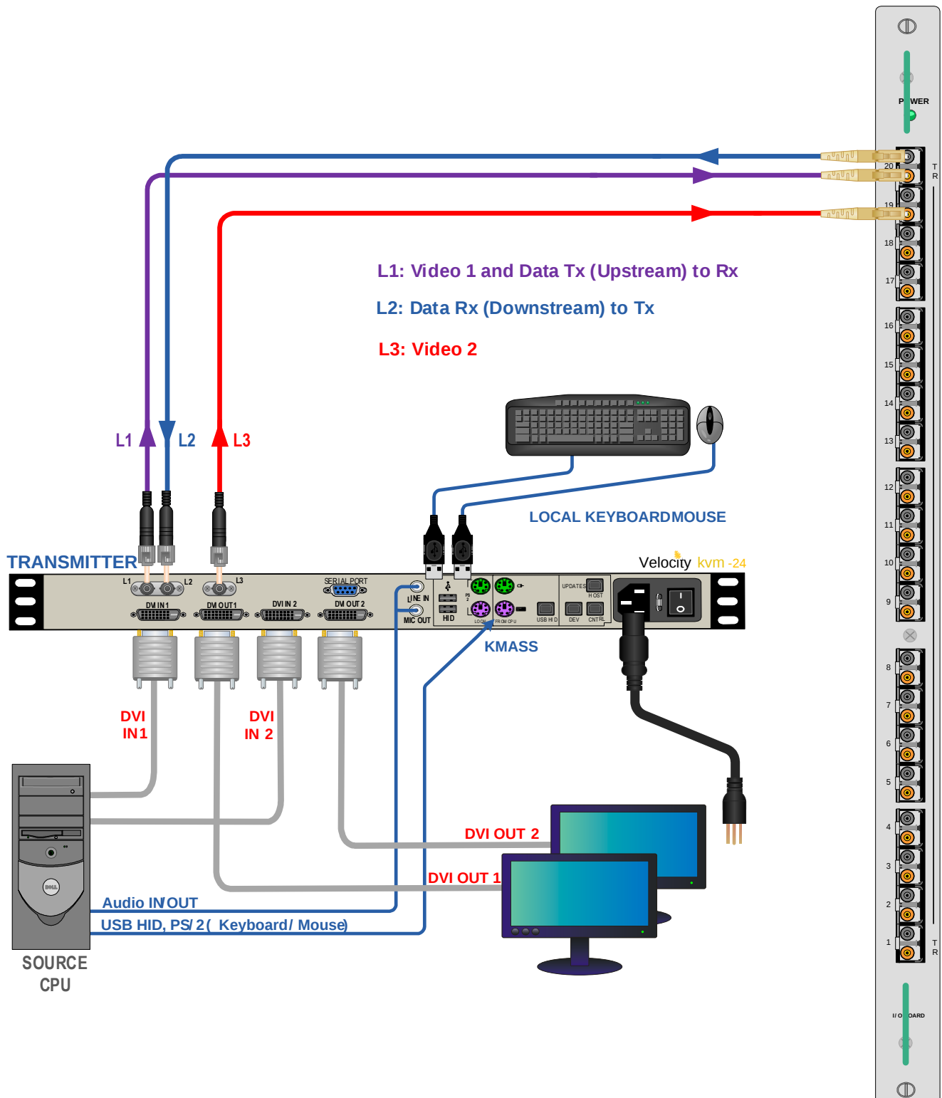
Connecting the Thinklogical VelocityKVM-24 Extender Transmitter to the VX160
