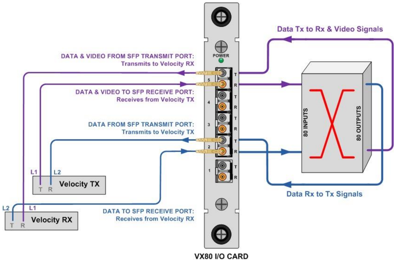
Figure 2: VX80 Input/Output Concept
