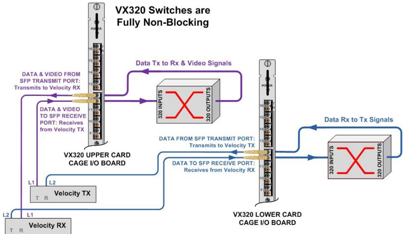
Figure 4: VX320 Input/Output Concept
