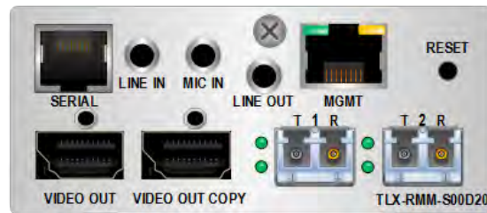
Modular Fiber Receiver with Audio & Serial
