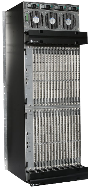
VX640 Router - Backpanel
