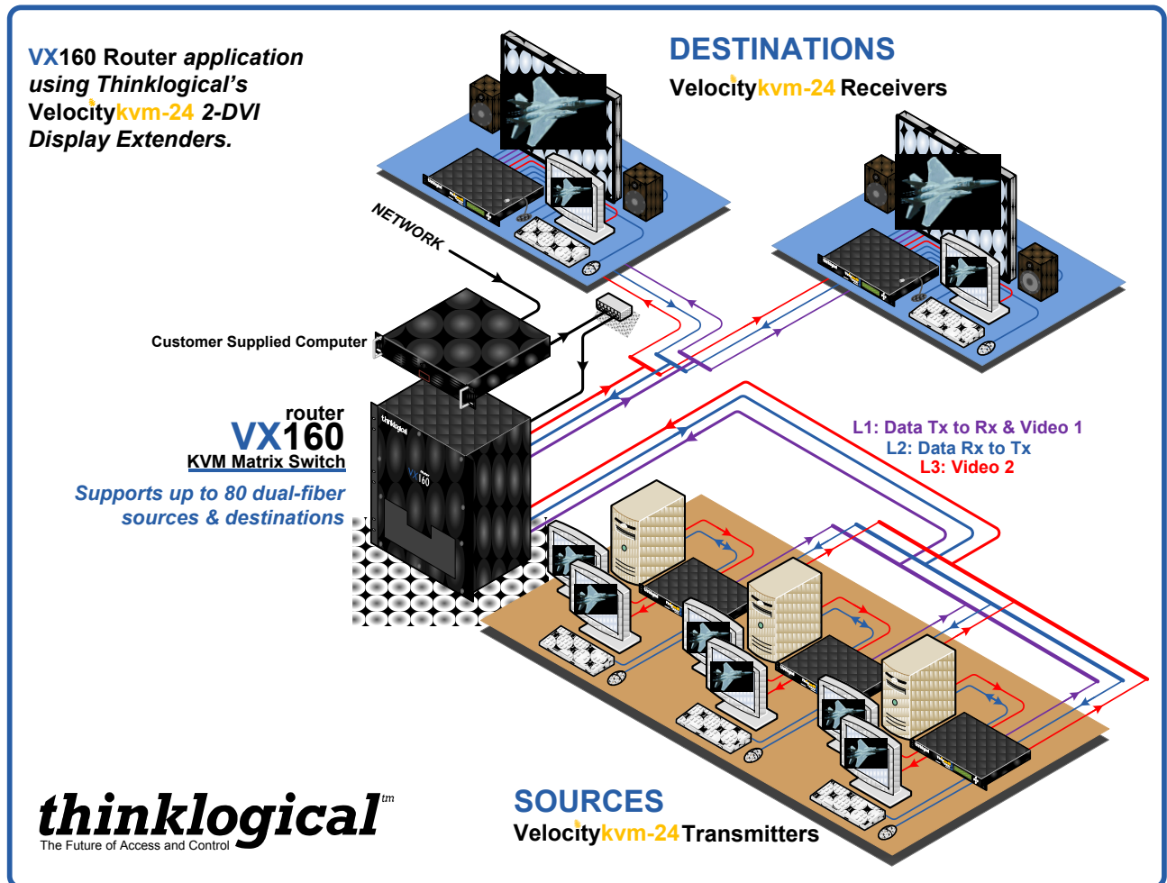
Figure 2a. Typical TOE VX160 Configuration
