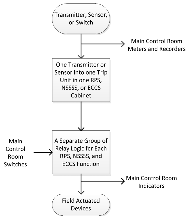
Figure 3-7. Existing RPS, N4S, and ECCS Architectural Detail
