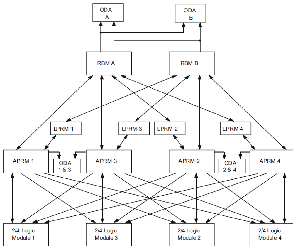
Figure 3-13. Neutron Monitoring Voter Structure (Reference 49)
